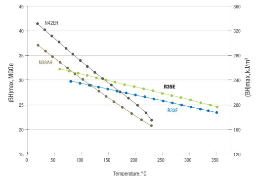
Comparison of Neo & SmCo as a function of temperature
